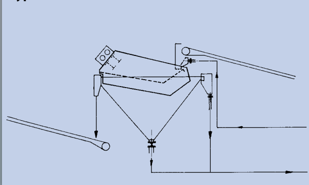
Typical flow-sheet
