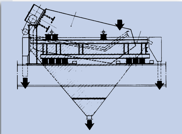
Typical flow-sheet
